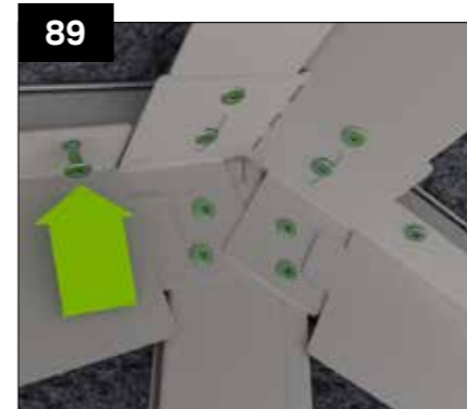
89 Secure gable panel on the inside through the previously attached angle WPCA/1, through the pre punched holes using the provided GPHS050 screws.
