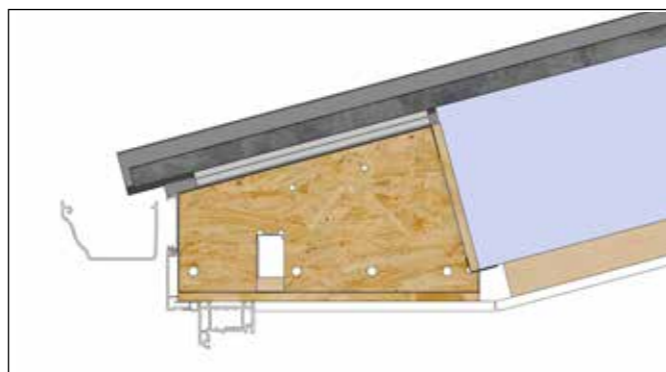
This image is the plaster line detail when at 15°.
