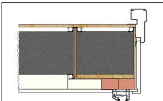
This image is showing the plaster line detail for a standard gable front. 44 x 70mm timber required above the gable frame.
