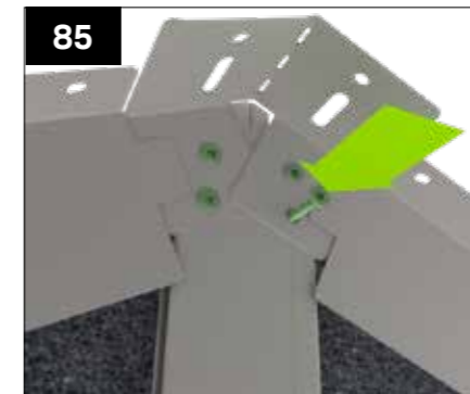
85 After gable wall is complete, attach the previously bent bracket to the apex of the wall and the internal angle brackets WPCA/1, aligning the upper angled faces with the top of the wall panels, using the GPHS050 screws through the pre punched holes into the vertical steel clips.
