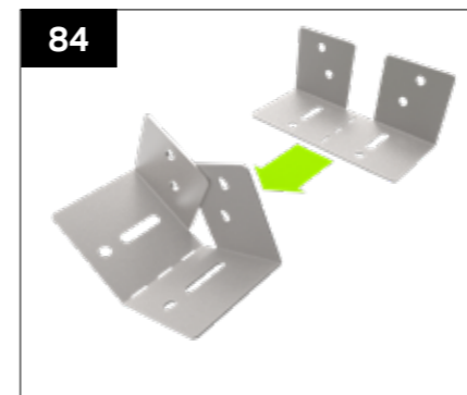
84 Bend provided gable ridge support bracket WPGR001 to the correct roof pitch along the perforated line.
