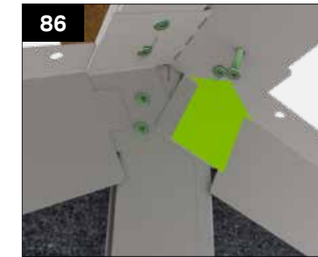
86 Position ridge and temporarily secure in bracket slot using the GPHS050 screws. Ensure level and walls are plumb, then tighten screw and add screws through final fix holes.
