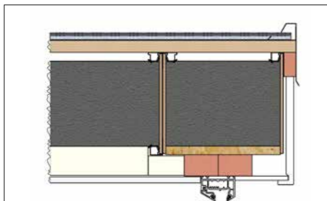
This image is showing the plaster line detail for an extended gable front. 44 x 70mm timber required above the gable frame.
