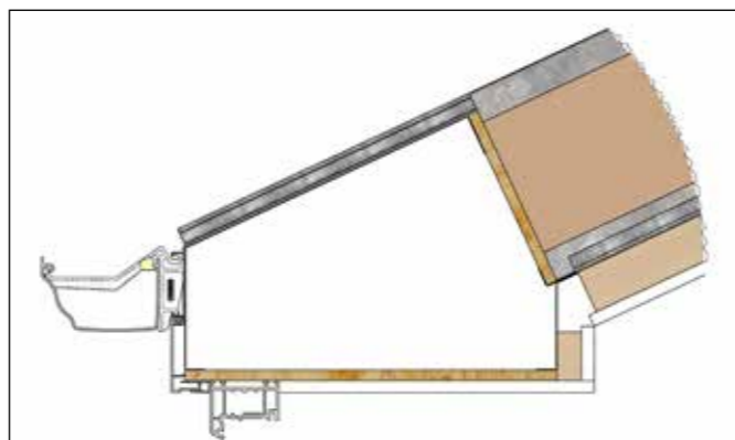
This image is the plaster line detail when 25°.
